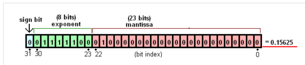
Fig. 2 Conversion to an IEEE Float
